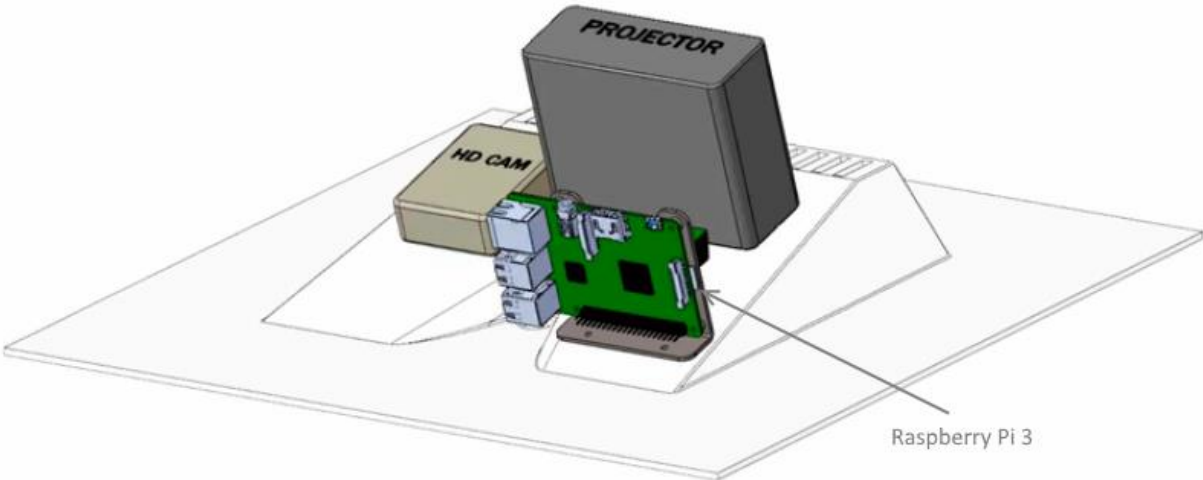
Image: projector, camera, and the motherboard inside color LED cover
